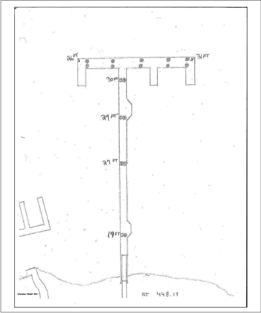
SITE SIX BOAT RAMP REPLACEMENT- DEPTH TO LAKE BED NO SCALE'
