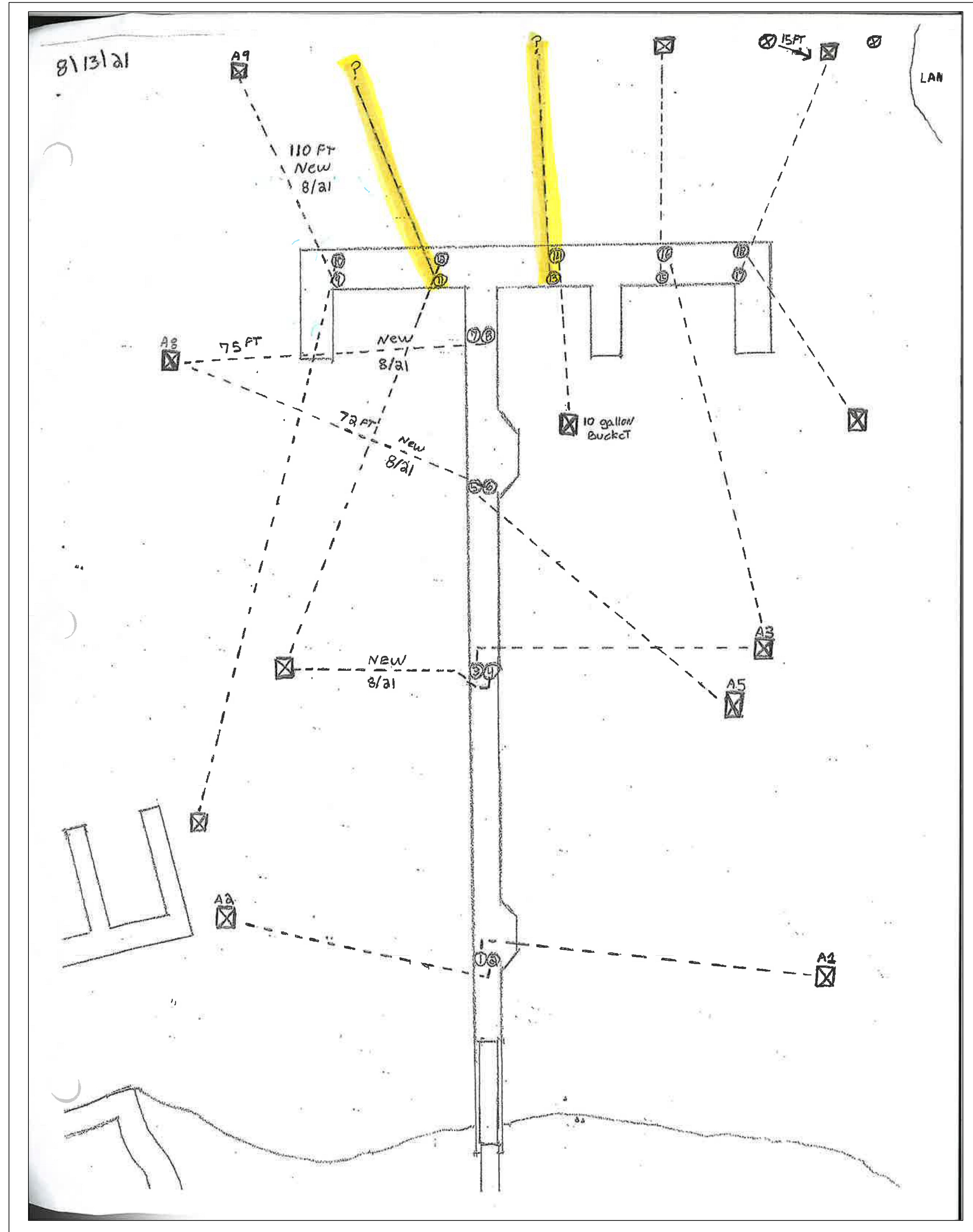
SITE SIX BOAT RAMP REPLACEMENT- ANCHORING SCHEMATIC NO SCALE'
